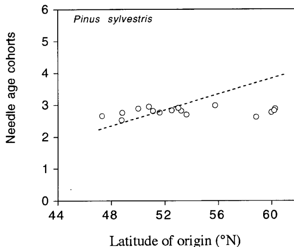
Figure 1. Mean number of needle age cohorts (annual age classes) in a common garden plantation (52° N) in Kórnik, Poland for 16 Pinus sylvestris (Scots pine) populations originating in low elevation sites across a latitudinal gradient. Standard deviation of number of needle age cohorts across blocks averaged about 10% of the mean values. There was no significant relationship ( P > 0.20 ) between needle longevity and latitude. The dashed line represents a hypothetical relationship between needle longevity and latitude of origin for these populations in this common garden environment if variation in needle longevity had a significant genotypic component (the exact position of the line has no meaning, given that this is an idealized conceptual hypothesis). This hypothesis is not supported.
